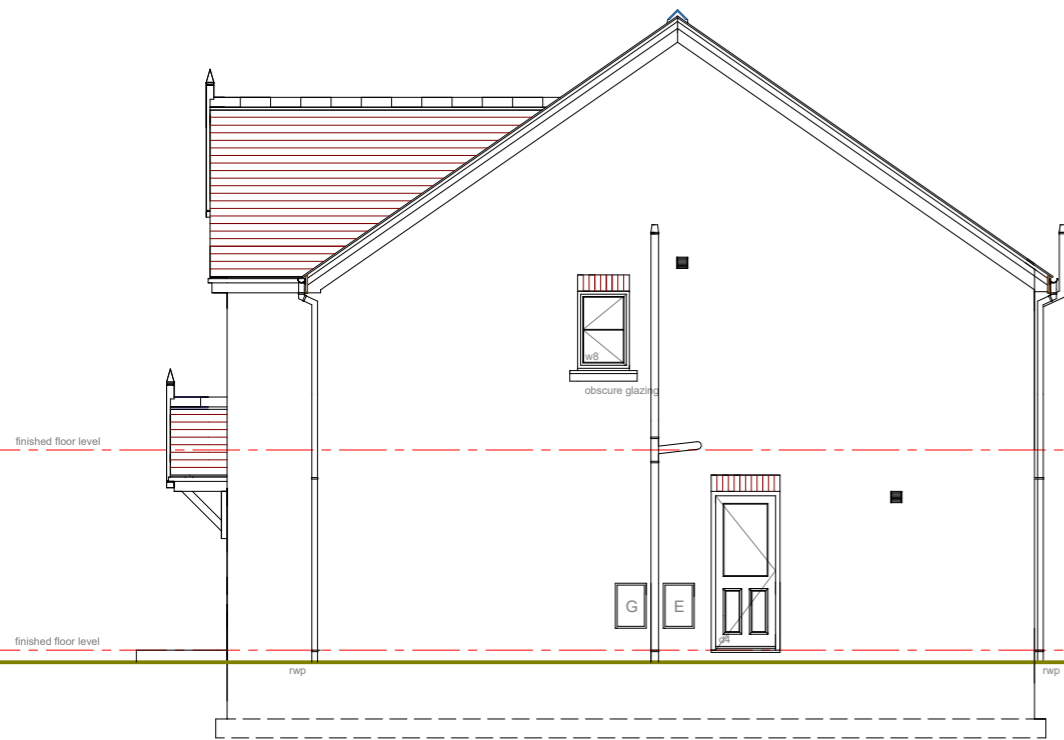
west elevation
