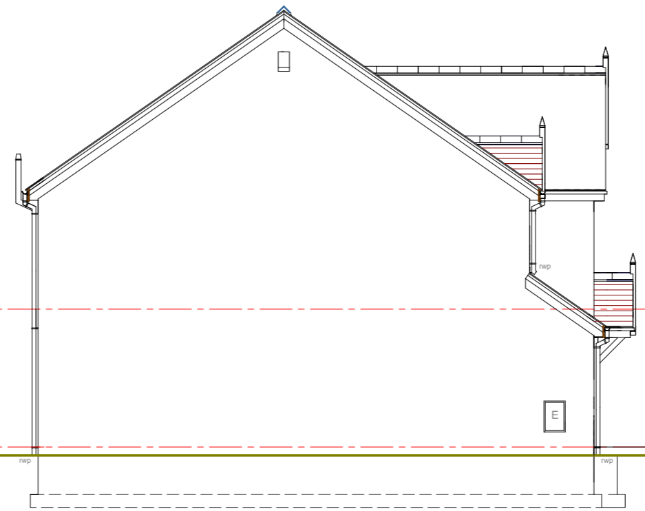
east elevation
