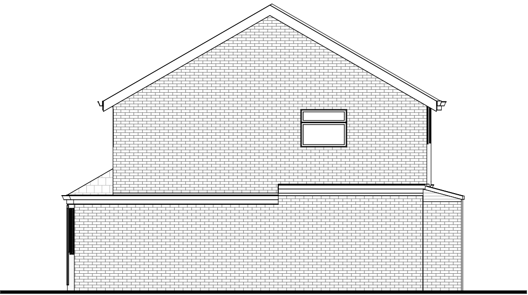
Existing South West Elevation 1 : 100
