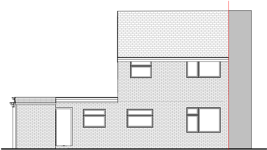
Existing South East Elevation 1 : 100
