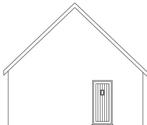
PROPOSED GARAGE
