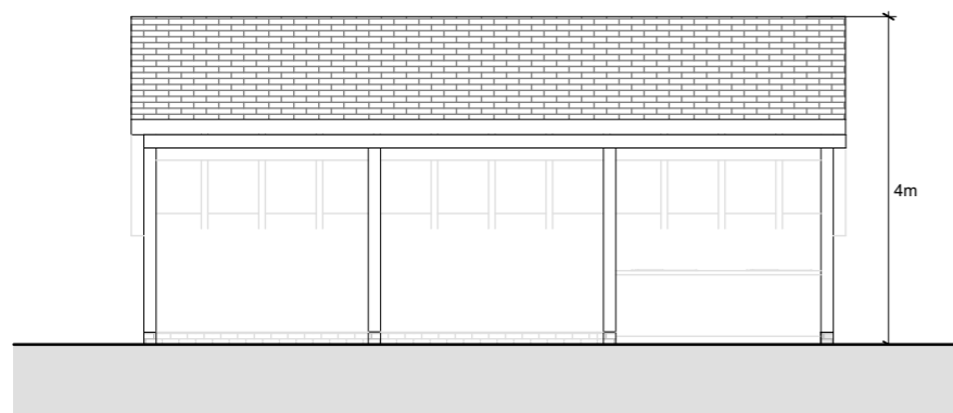
Multi- Purpose Activity Centre Elevation North 1:100
