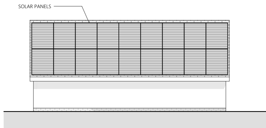
E-30 Multi- Purpose Activity Centre South Elevation 1:100
