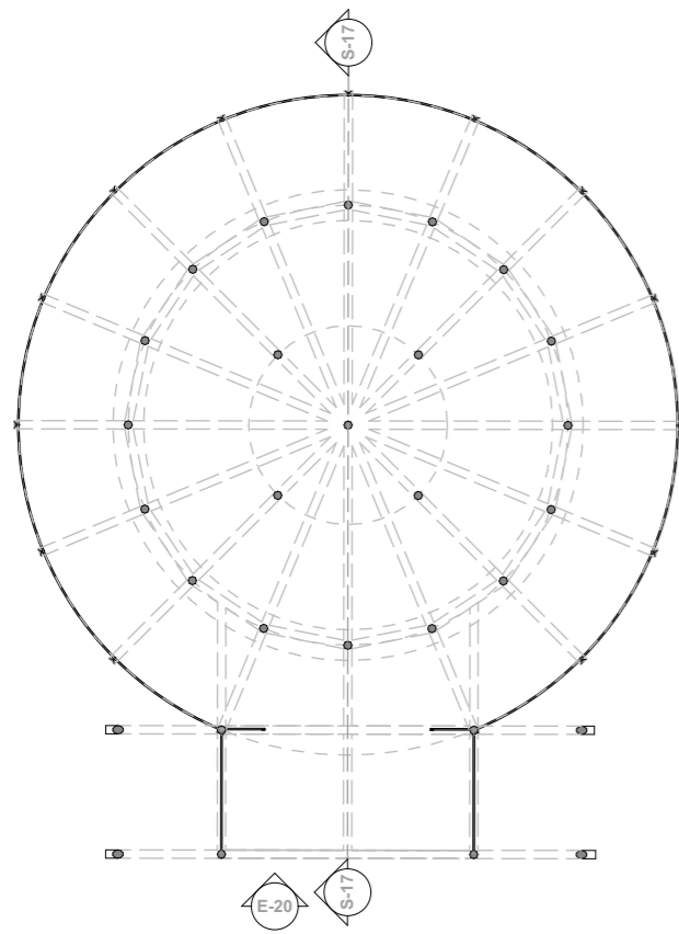
1. GROUND FLOOR 1:100
