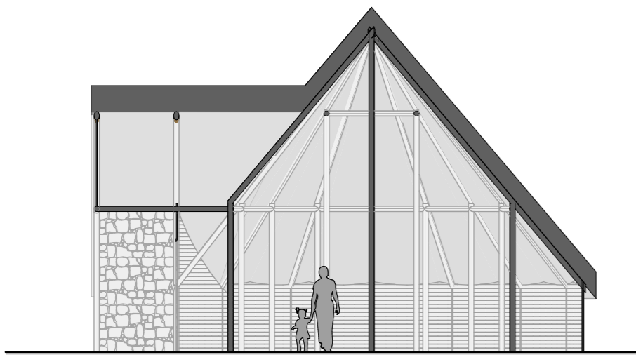
S-17 Type A Iron-Age Roundhouse Section 1:100
