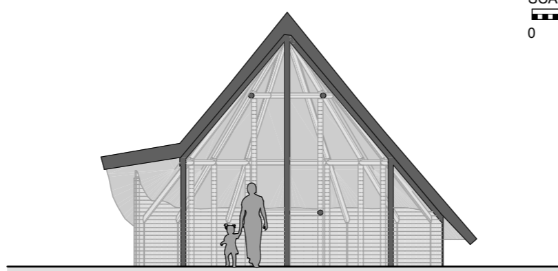
S-22 Type B Iron-Age Roundhouse Section 1:100
