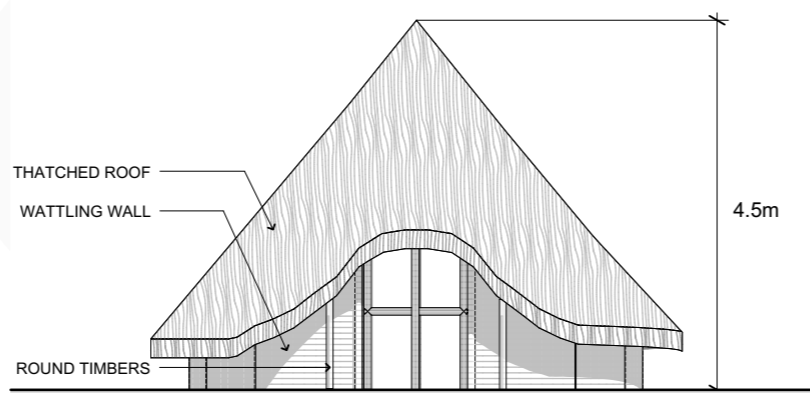
E-21 Type B Iron-Age Roundhouse Elevation 1:100
