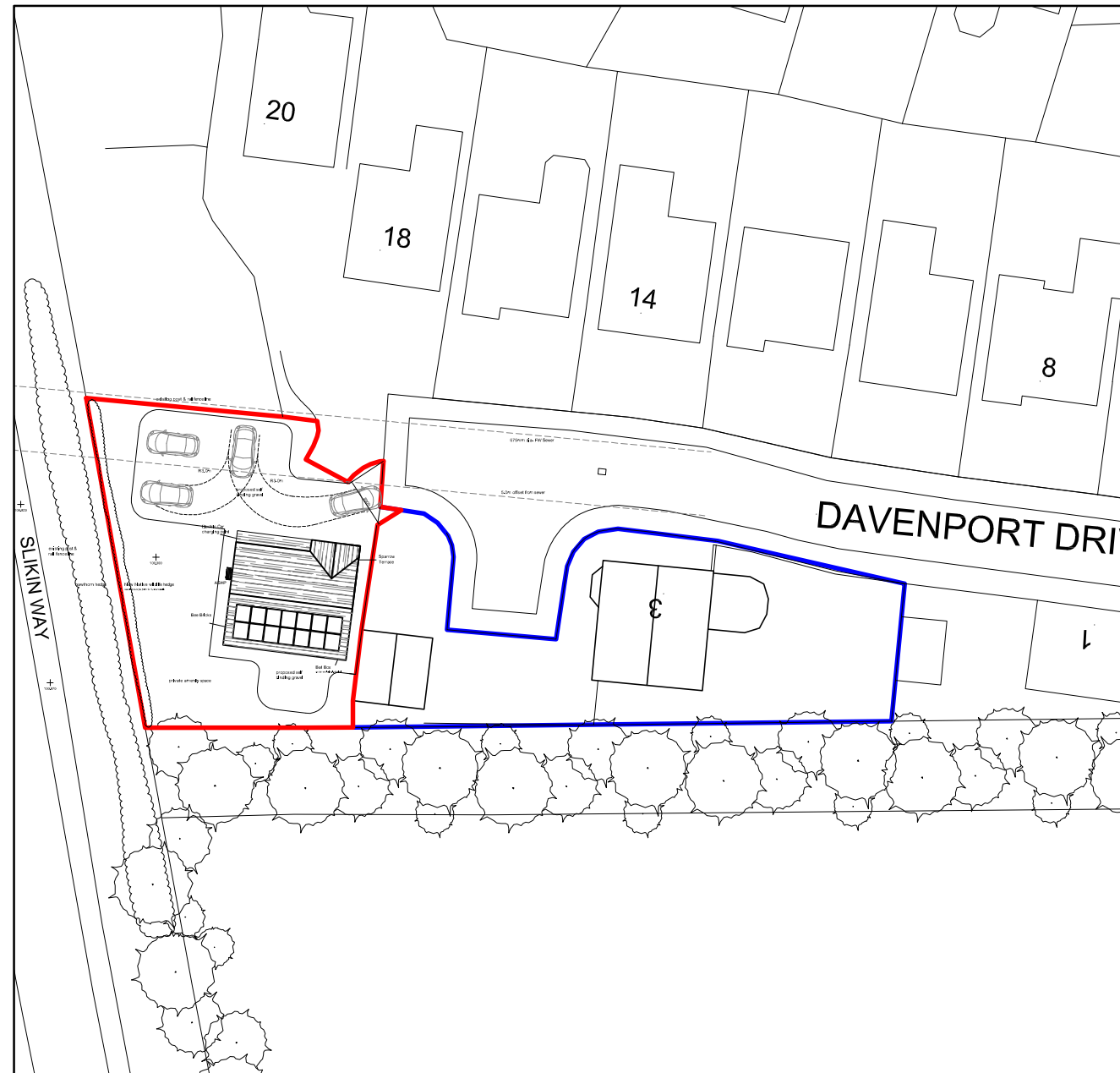
Block Plan 1:500
