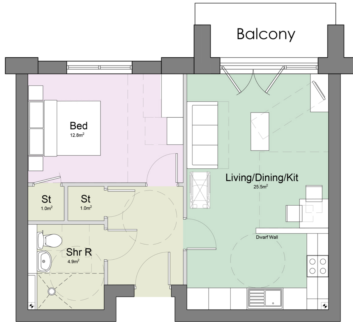
1 Bed 2 Person Apartment - 52.2 sqm NDSS Min Area - 50 sqm NDSS Min Storage - 1.5 sqm NDSS Min Bed Area & Width - 11.5 sqm / 2.75m
