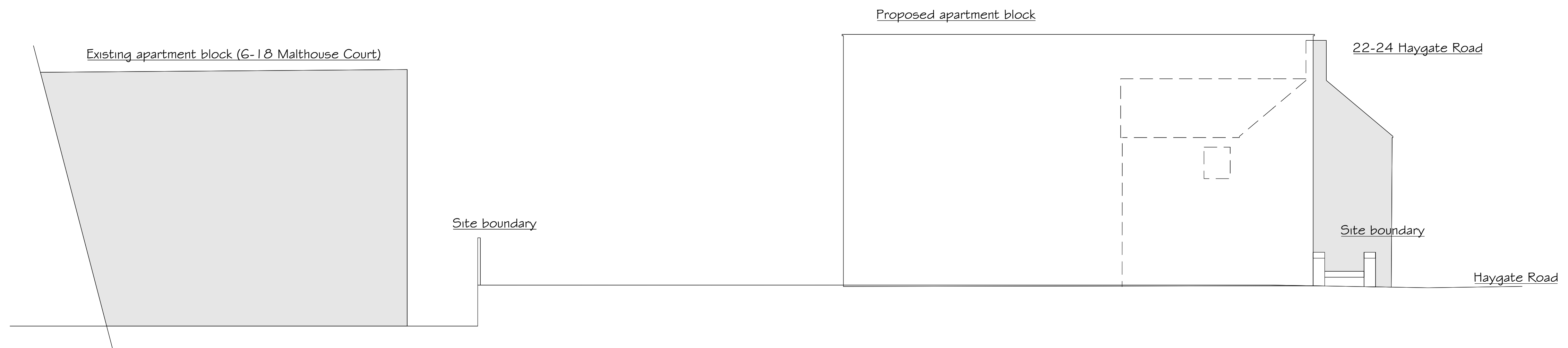
Site Cross Section B-B
