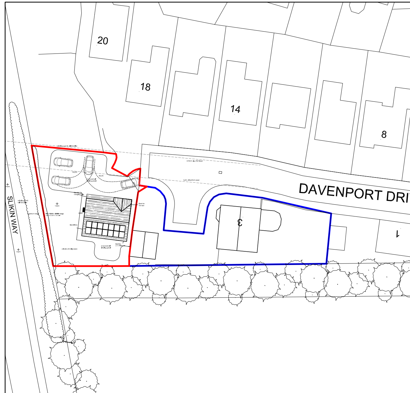
Block Plan 1:500
